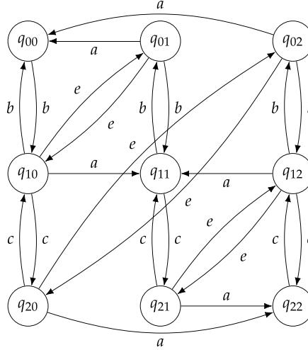
FIGURE 3. A non-synchronizing permutation-primitive DFA from [13] with a letter of rank 3. If the action of a letter x \in \{a, b, c, e\} at some state is not shown, then the loop labeled x is assumed.
